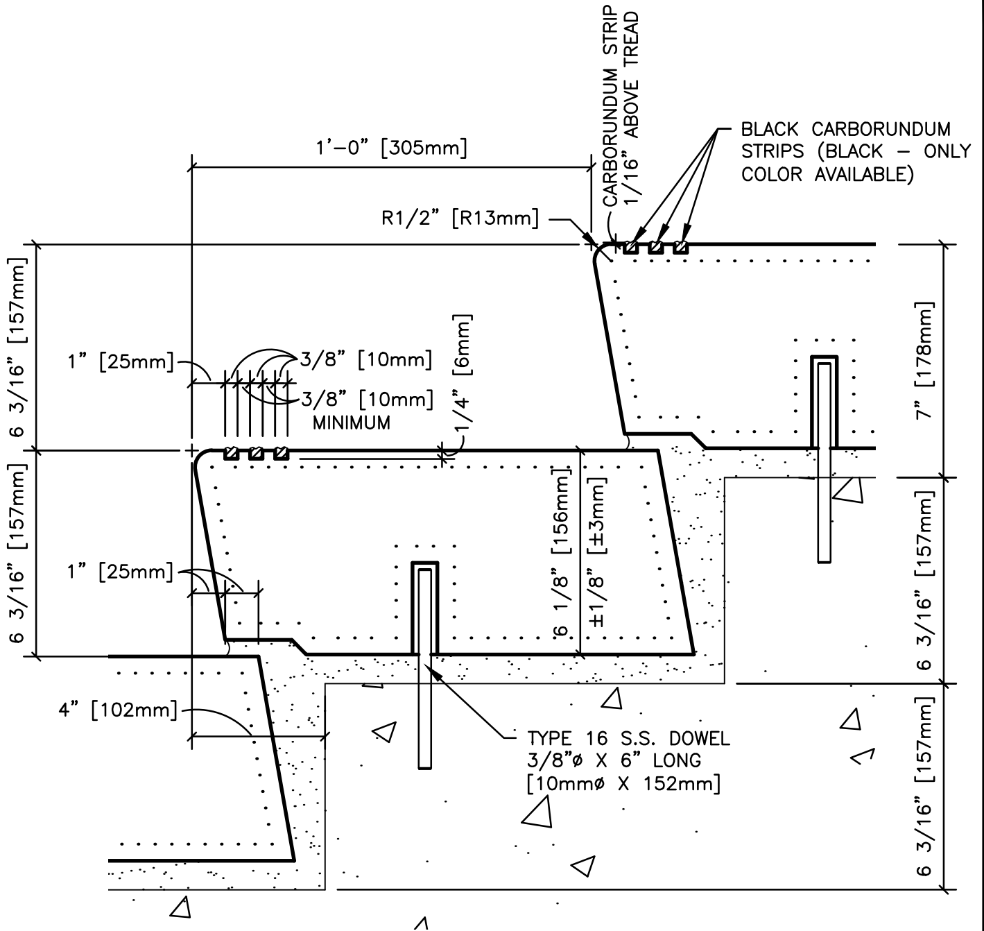
STAIR TREAD CUBIC WITH CARBORUNDUM
