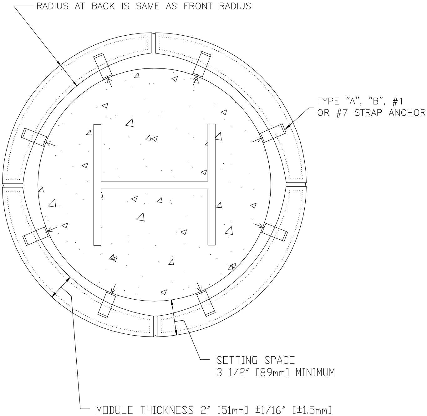
PLAN - ROUND COLUMN COVER
